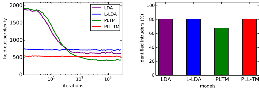
(a) Comparison of the held-out perplexity (lower values are better) as a function of iterations. (b) Comparison of the semantic coherence (word intrusion) of the generated topics.
