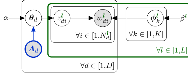
Fig. 1: The PLL-TM in plate notation. Random variables are represented by nodes. Shaded nodes denote the observed words and labels, bare symbols indicate the fixed priors \alpha and \beta^l . Directed edges between the nodes then define conditional probabilities, where the child node is conditioned on its parents. The rectangular plates indicate replication over data-points and parameters. Colors indicate the parts which are inherited from L-LDA ( blue ) and PLTM ( green ). Black is used for the LDA base.
