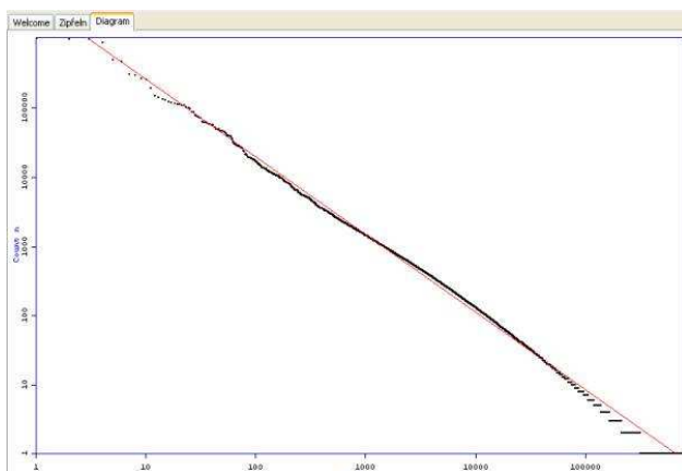
Figure 7: A fitted Zipfian distribution
